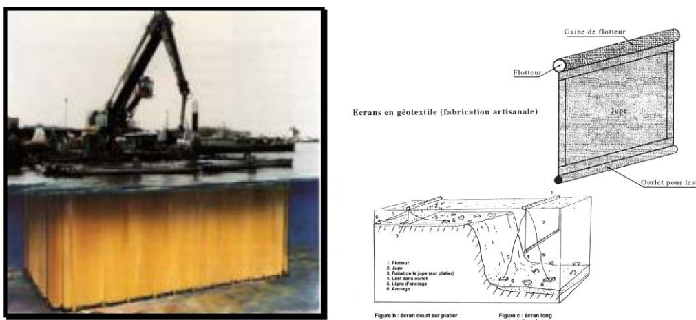
Figure 125: Ecran anti-sédimentaire
